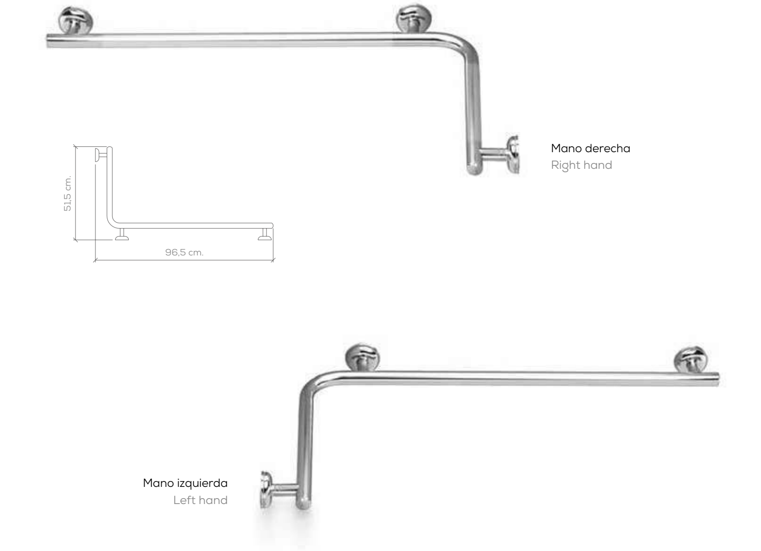
ASIDERO angular 90° a dos paredes Inox. 18/10 18/10 stainless steel 90° angled handrail with 2-wall mounting for shower stalls
