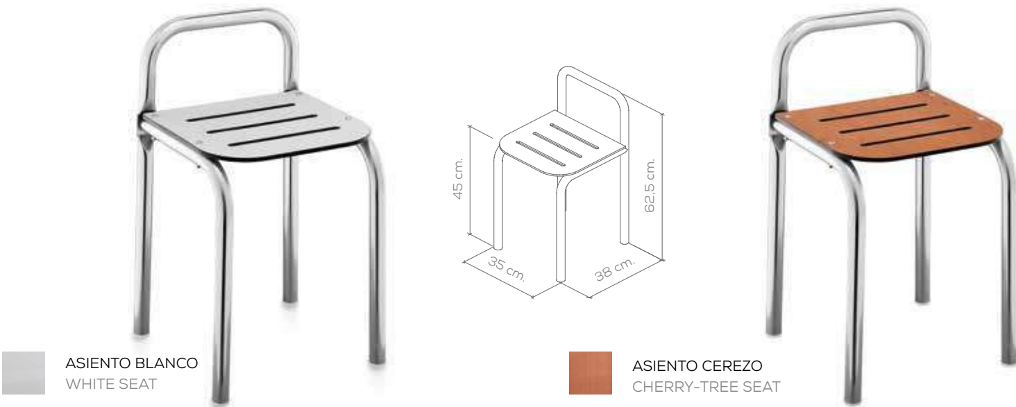
BANQUETA con respaldo de tubo Inox. 18/10 18/10 stainless steel stool with tubular backrest
